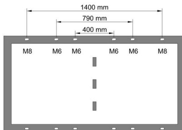
Bolt locations on the module
