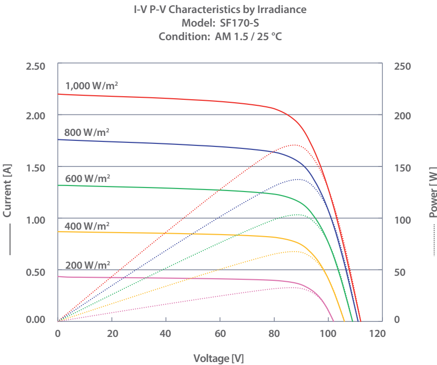
Typical characteristics
