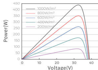
Power-Voltage Curves (440W)
