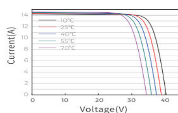
Current-Voltage Curves (440W)
