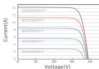
Current-Voltage (440W)
