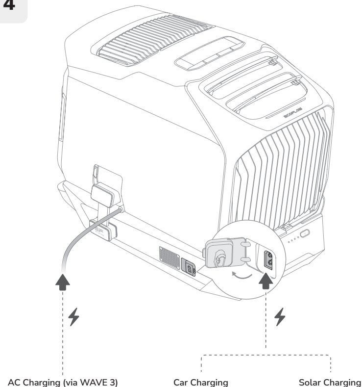
AC Charging (via WAVE 3)
